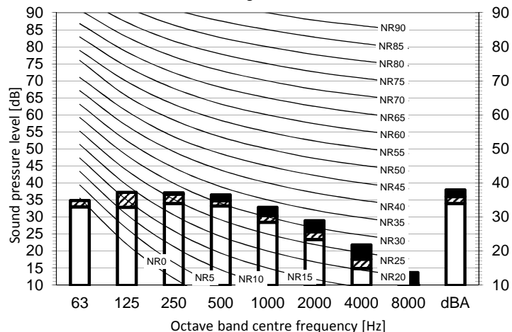
Heating mode
