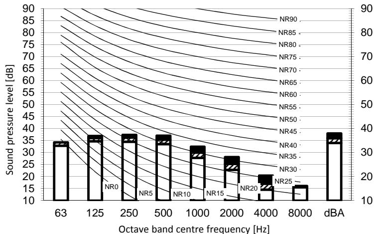
Cooling mode
