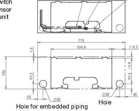
Standard location of holes in the wall
